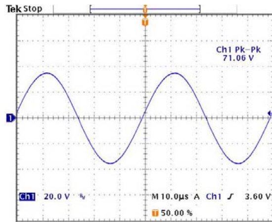
20kHz sine into 8 \Omega load, G = -10 , C_c = 100pF
