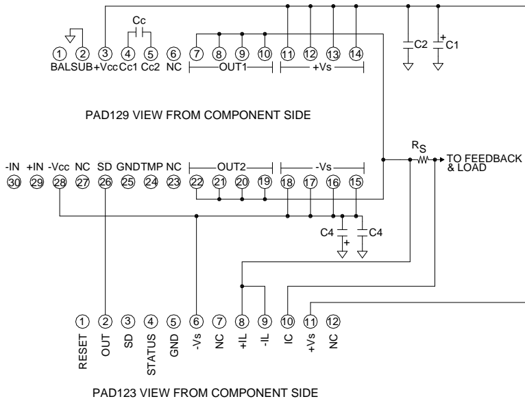
FIGURE 2. TYPICAL PAD129 CONNECTIONS TO PAD123 ACCESSORY MODULE
