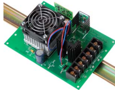
PAD129 mounted in EVAL128 evaluation kit with accessory modules.
