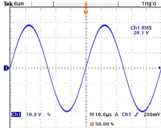
20kHz into 4Ω load, G=-10, Cc=100pF
