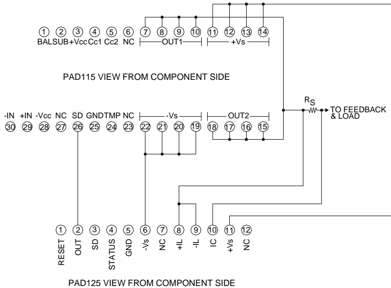
FIGURE 2. TYPICAL PAD115 CONNECTIONS TO PAD125 ACCESSORY MODULE
